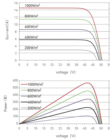
I-V curve
