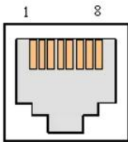
RJ45 Socket
